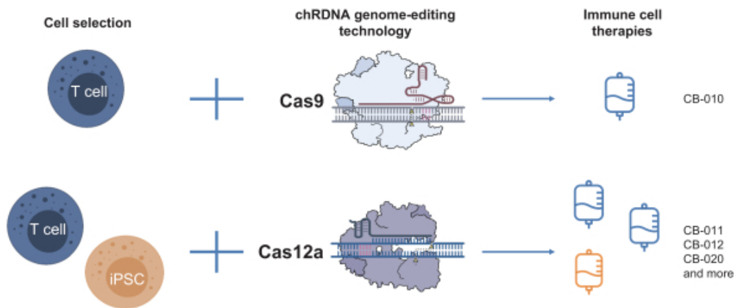
Figure 5. We use Cas9 and Cas12a in the development of our allogeneic cell therapies.
